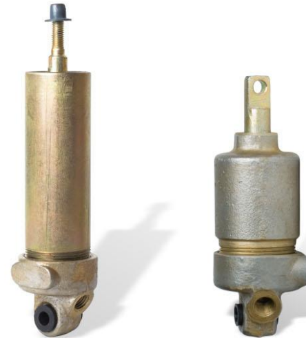
Pneumatic Cylinder 35x65 100-3570210
